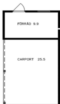
PLAN 35.4 Kvm
