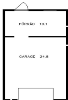
PLAN 35.3 Kvm
